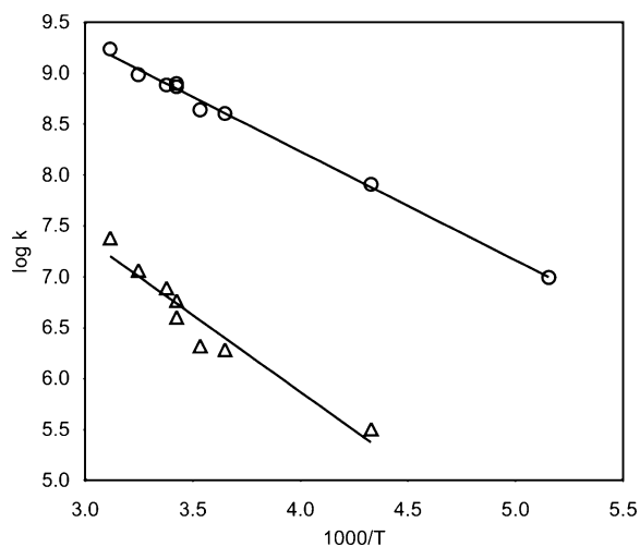
FIGURE 1. Arrhenius functions for fragmentation of radical 2 → 1 (Δ) and 2 → 3 (○).
